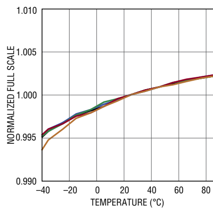
Normalized Full Scale vs Temperature, External Reference, 5 Units
