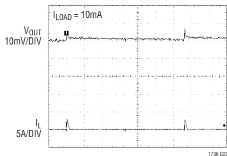
V_{OUT(RIPPLE)} (Synchronized)
