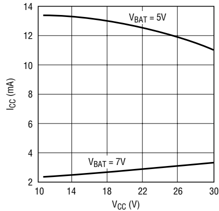
I_{\text{CC}} vs V_{\text{CC}} (8.4V Version)
