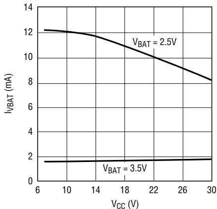
I_{\text{VBAT}} vs V_{\text{CC}} (4.2V Version)
