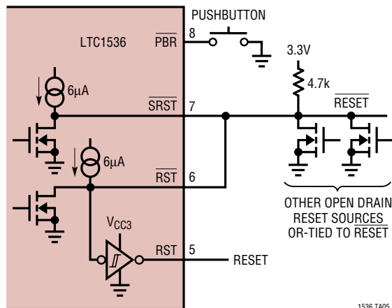
\overline{\text{SRST}} Tied to \overline{\text{RST}} and OR-Tying Other Sources to \overline{\text{RST}} to Generate Reset and Reset
