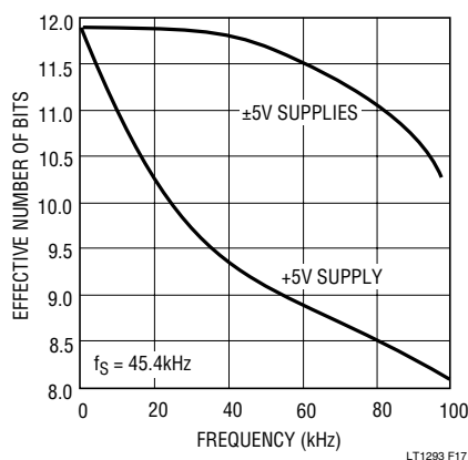
Figure 17. LTC1294 ENOB vs Input Frequency
