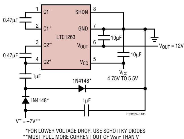
Dual Supply Voltage Output at 12V and -7V
