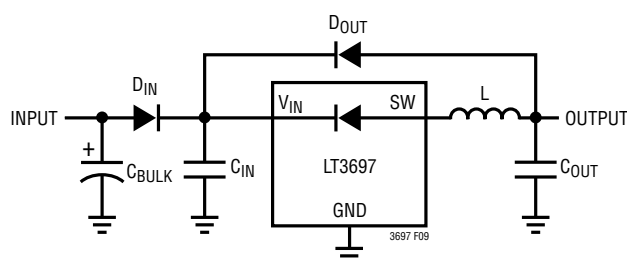
Figure 9. Diodes D_{IN} and D_{OUT} Prevent High Current Flow in the LT3697 if the Input Is Grounded or Floating and the Output Is Pulled High.
