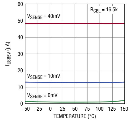
USB5V Current
