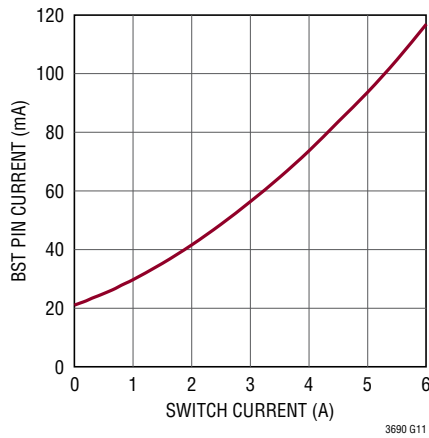
BST Pin Current vs I_{SW}
