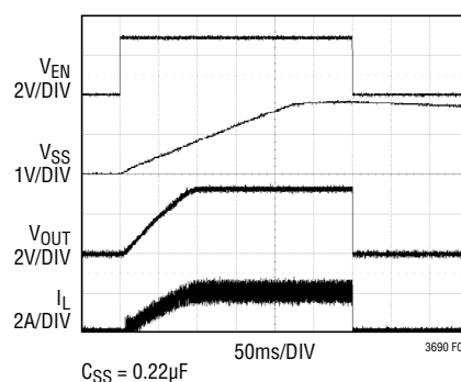
Figure 7. Soft-Start Ramp
