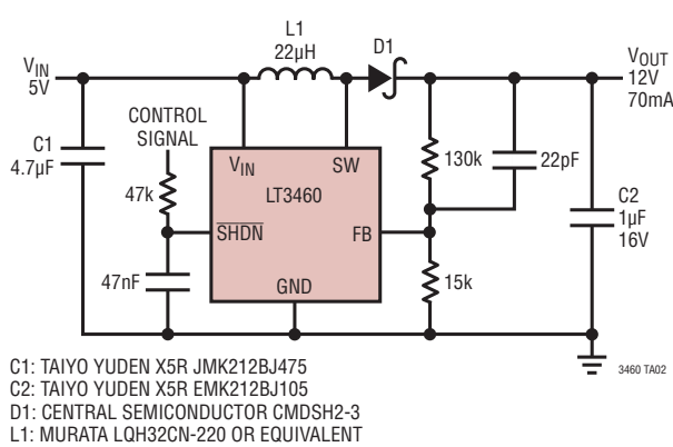
5V to 12V with Soft-Start Circuit
