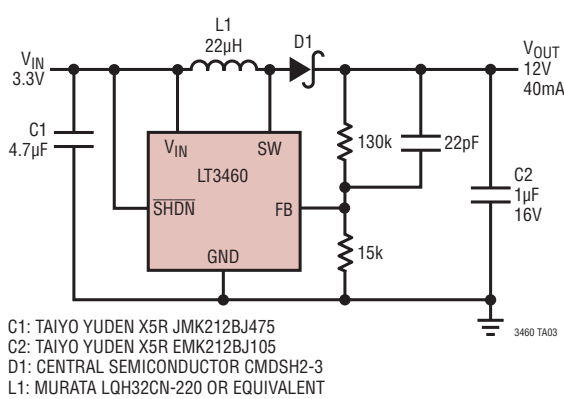
5V to 12V Step-Up Converter
