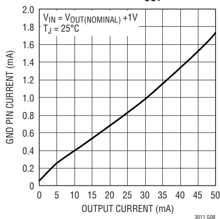
GND Pin Current vs I_{\text{OUT}}
