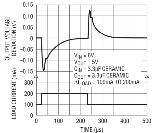
Transition Response
