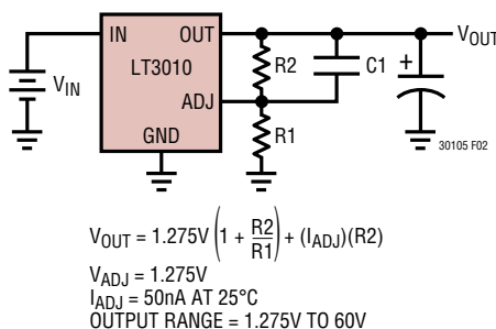
Figure 2. Adjustable Operation
