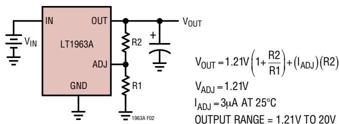
Figure 2. Adjustable Operation
