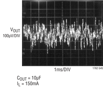
LT1762-5 10Hz to 100kHz Output Noise C_{BYP} = 100pF
