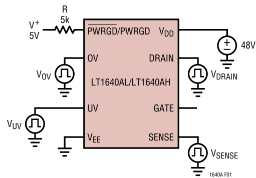
Figure 1. Test Circuit
