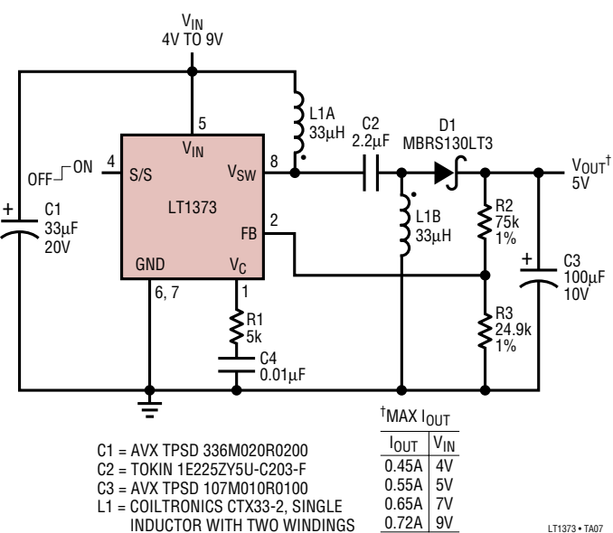
Two Li-Ion Cells to 5V SEPIC Converter
