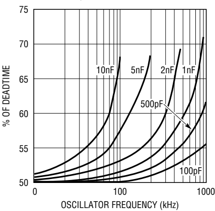
Output Deadtime vs Oscillator Frequency – LT1241, LT1243, LT1245
