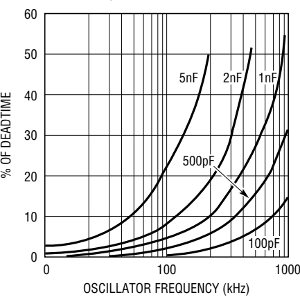
Output Deadtime vs Oscillator Frequency – LT1242, LT1244
