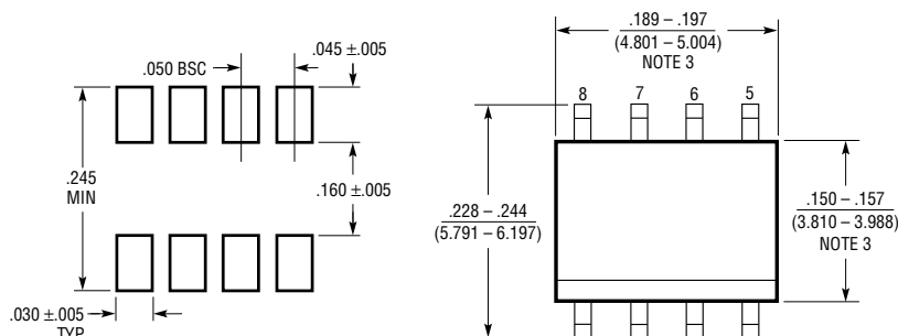
RECOMMENDED SOLDER PAD LAYOUT
