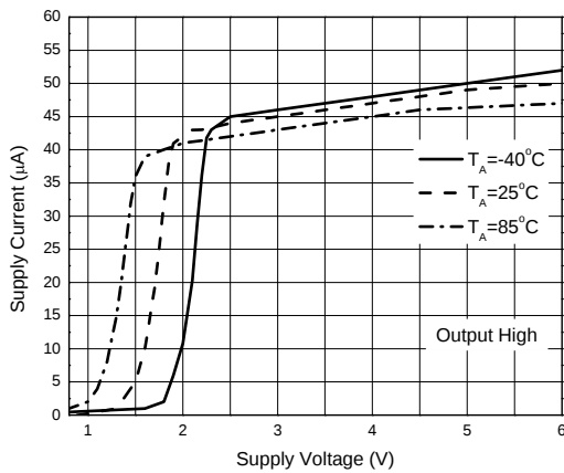
Supply Current vs. Supply Voltage (LMV331)
