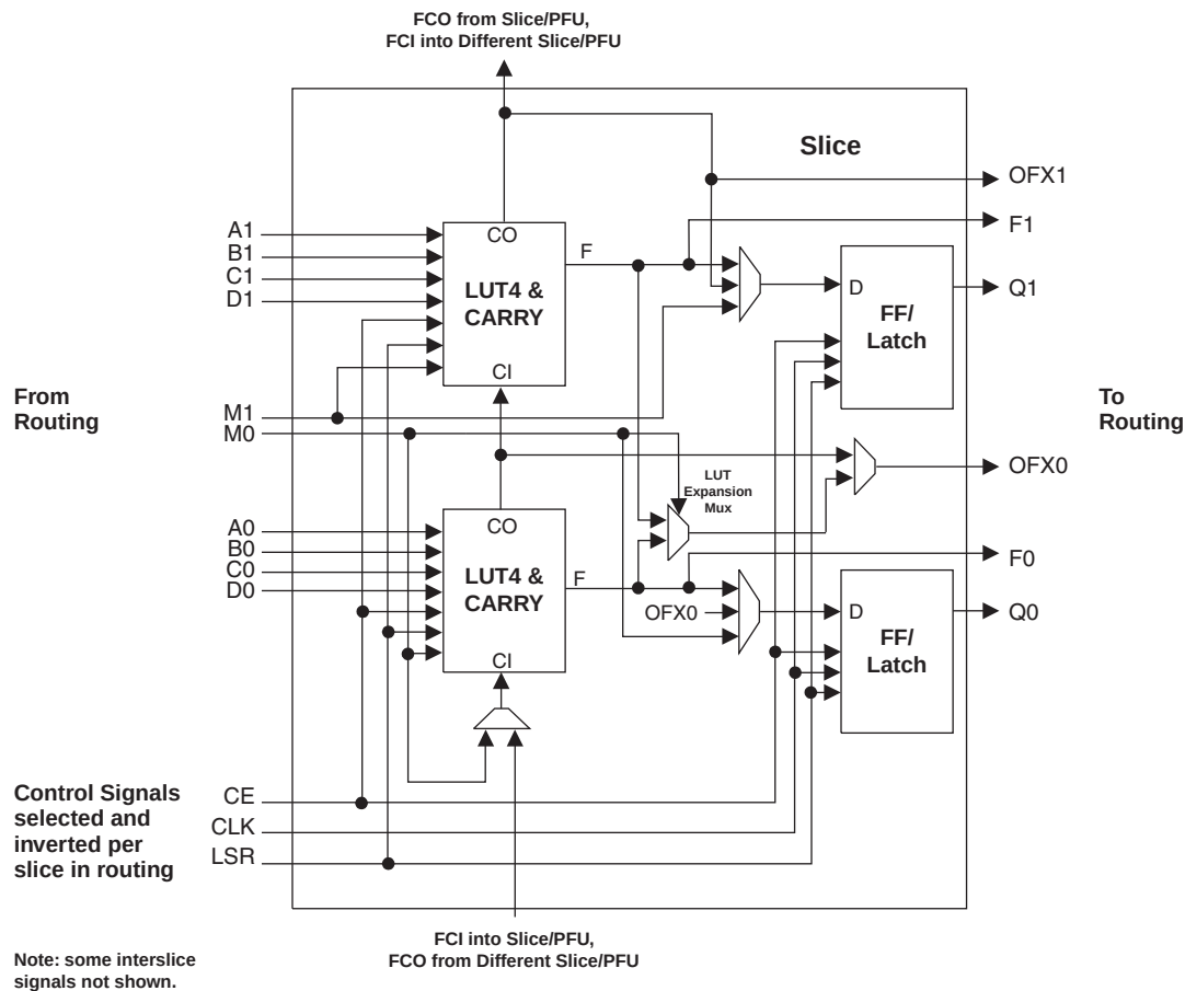
Figure 2-3. Slice Diagram
