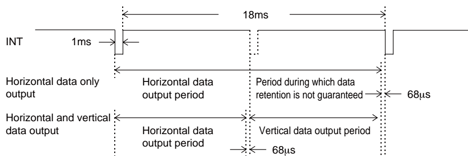
Figure 2 External Interface - Basic Timing
