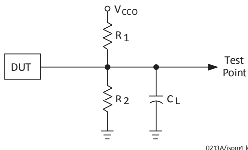
Figure 32.1. Output Test Load, LVTTTL and LVCMOS Standards
