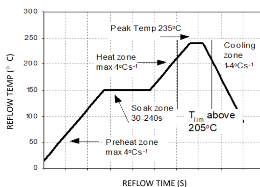
Figure 20. Recommended Reflow Profile for Sn/Pb solder.
