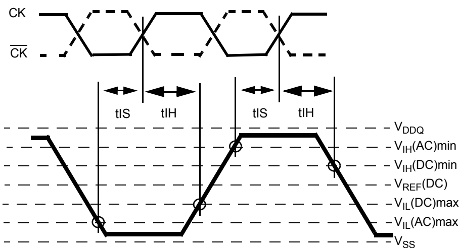
Figure 21. Differential input waveform timing - t_{IS} and t_{IH}
