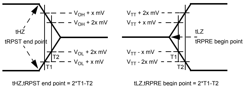
Figure 19. Method for calculating transitions and endpoints
