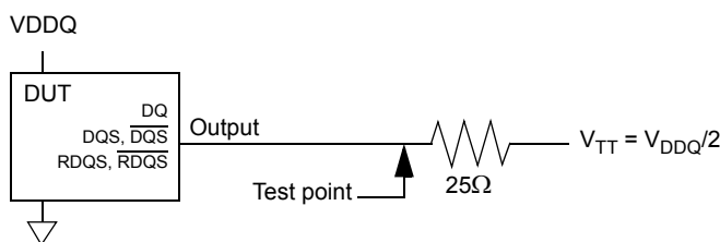
Figure 2. Slew Rate Test Load
