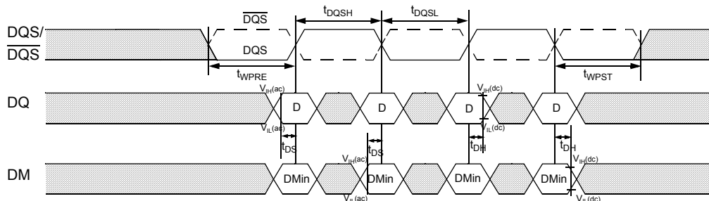
Figure 3. Data Input (Write) Timing
