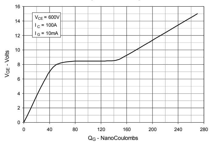
Fig. 8. Gate Charge
