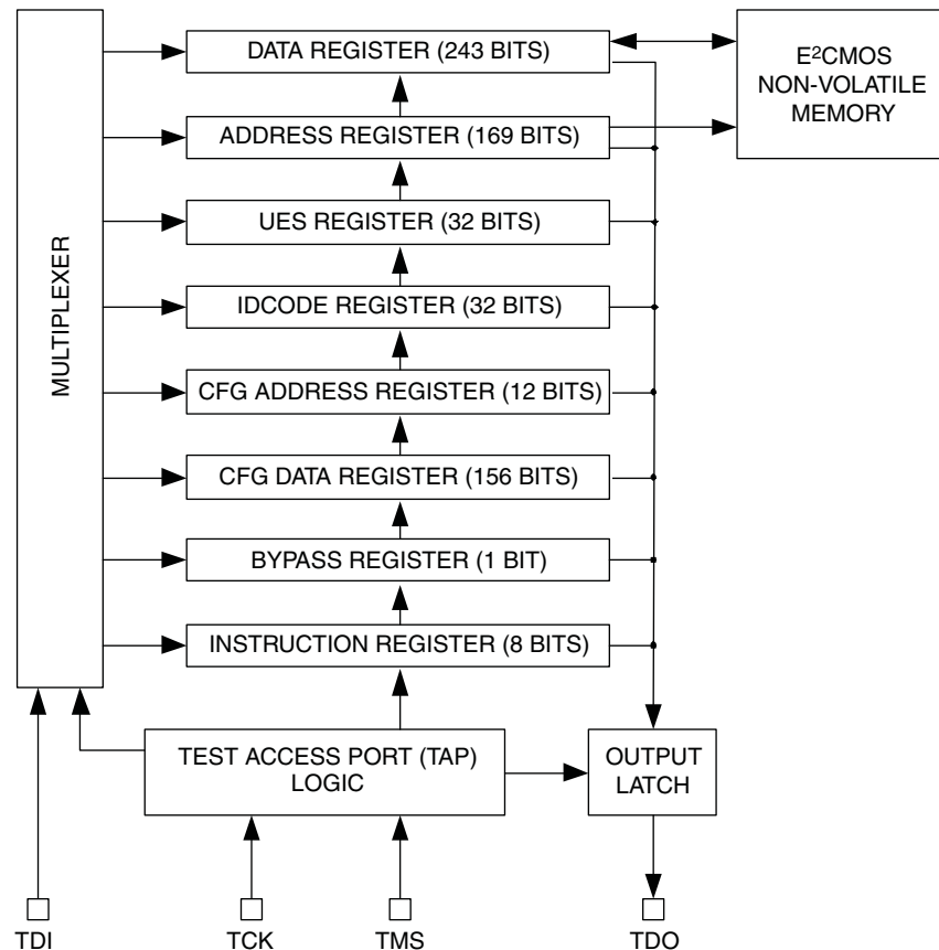
Figure 39. ispPAC-POWR1220AT8 TAP Registers
