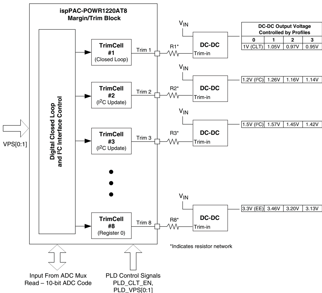
Figure 16. ispPAC-POWR1220AT8 Trim and Margin Block
