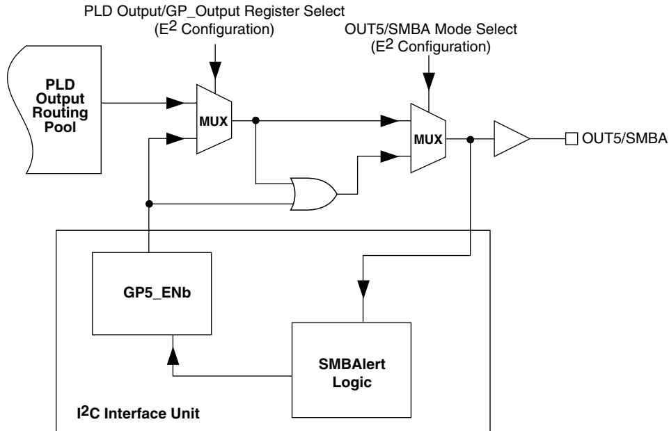
Figure 32. ispPAC-POWR1220AT8 SMBAlert Logic
