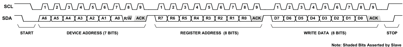
Figure 23. I 2 C Write Operation
