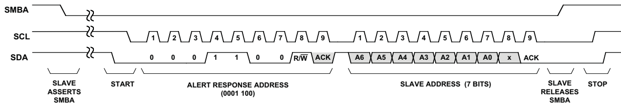
Figure 33. SMBAlert Bus Transaction
