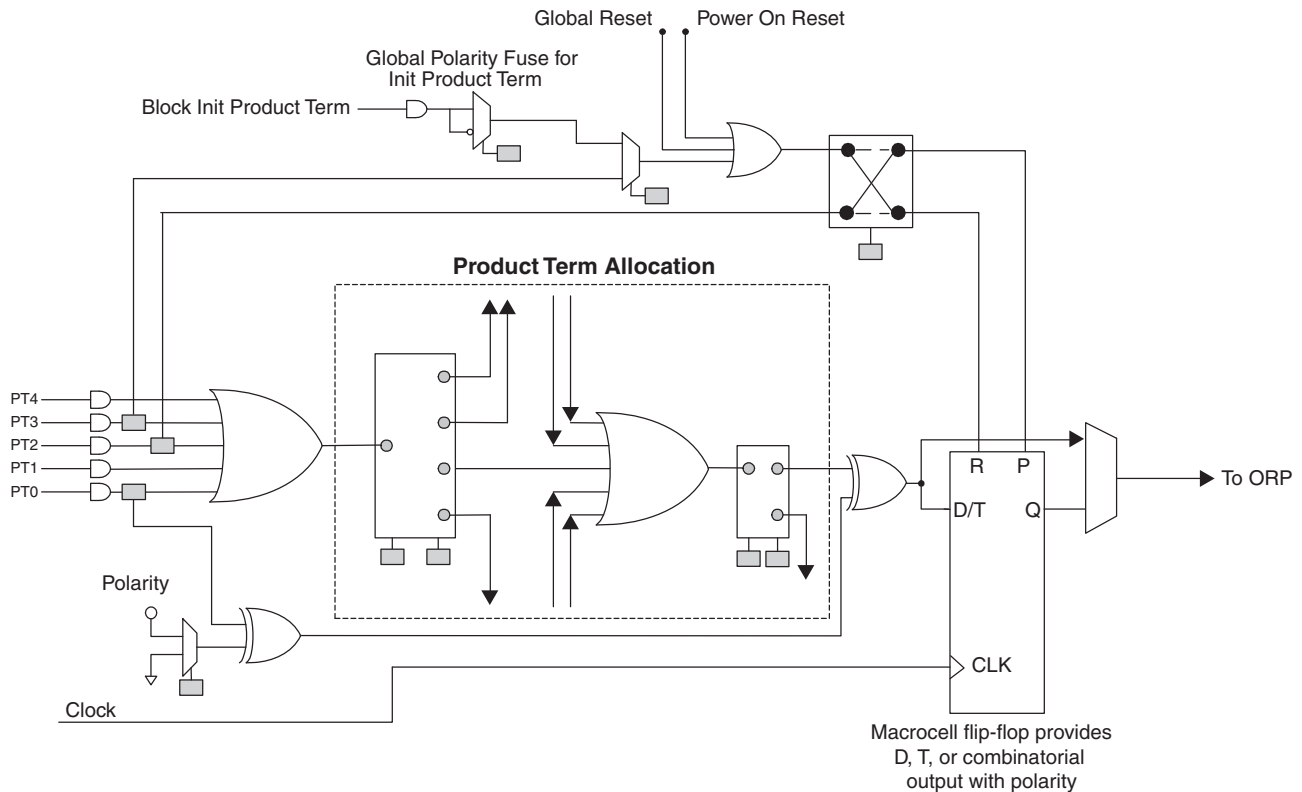
Figure 11. ispPAC-POWR1220AT8 Macrocell Block Diagram
