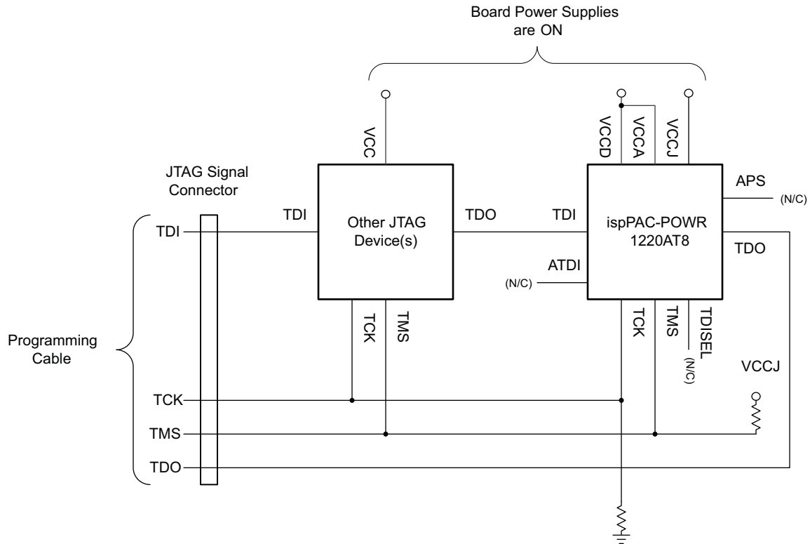
Figure 35. ispPAC-POWR1220AT8 JTAG Interconnection Configuration Diagram
