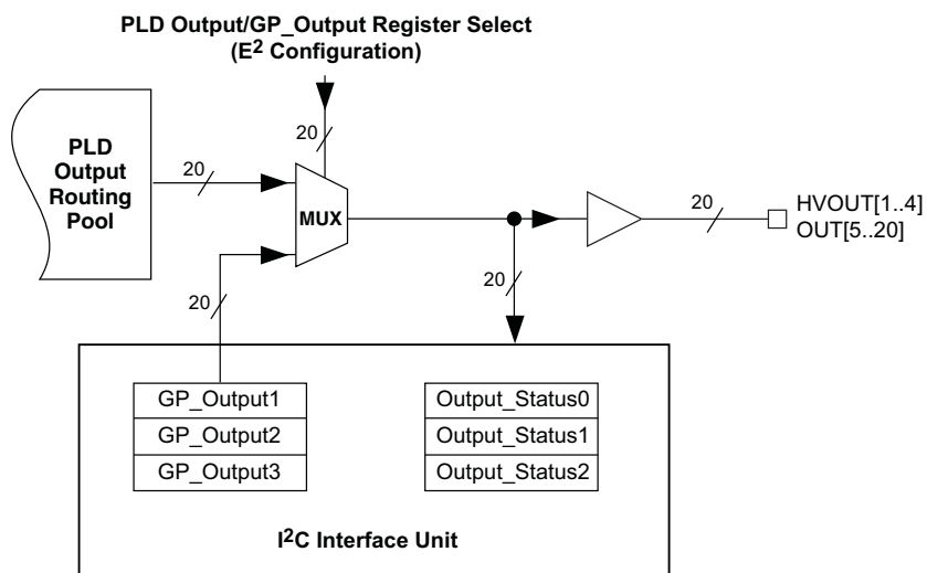
Figure 28. I 2 C Output Monitor and Control Logic
