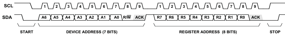
Figure 24. I 2 C Read Operation
