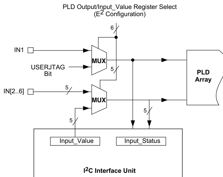
Figure 27. I 2 C Digital Input Interface
