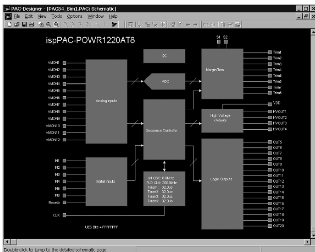
Figure 34. PAC-Designer ispPAC-POWR1220AT8 Design Entry Screen
