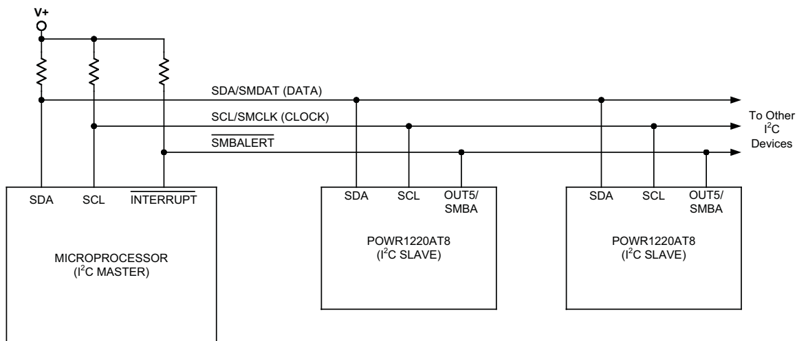
Figure 22. ispPAC-POWR1220AT8 in I 2 C/SMBUS System
