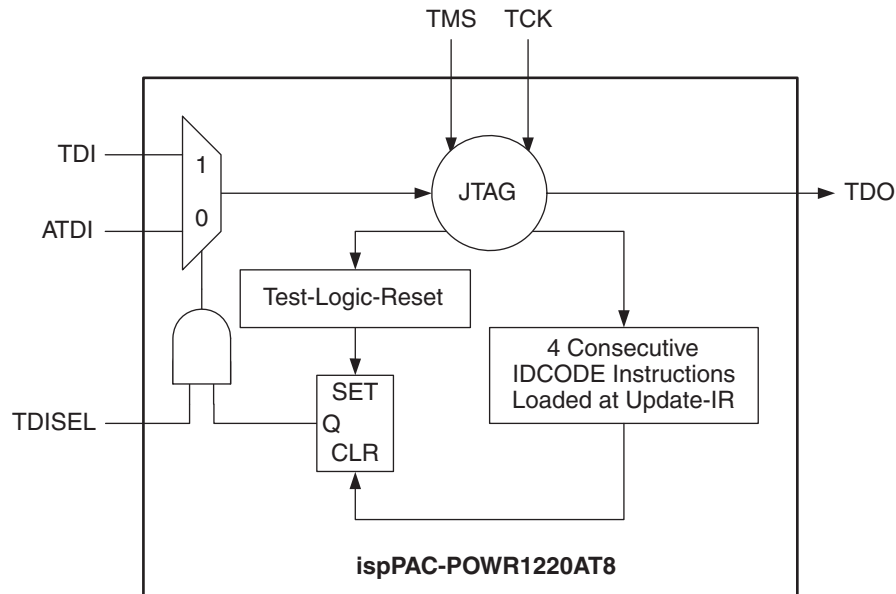
Figure 37. ispPAC-POWR1220AT8 TDI/ATDI Pin Selection Diagram
