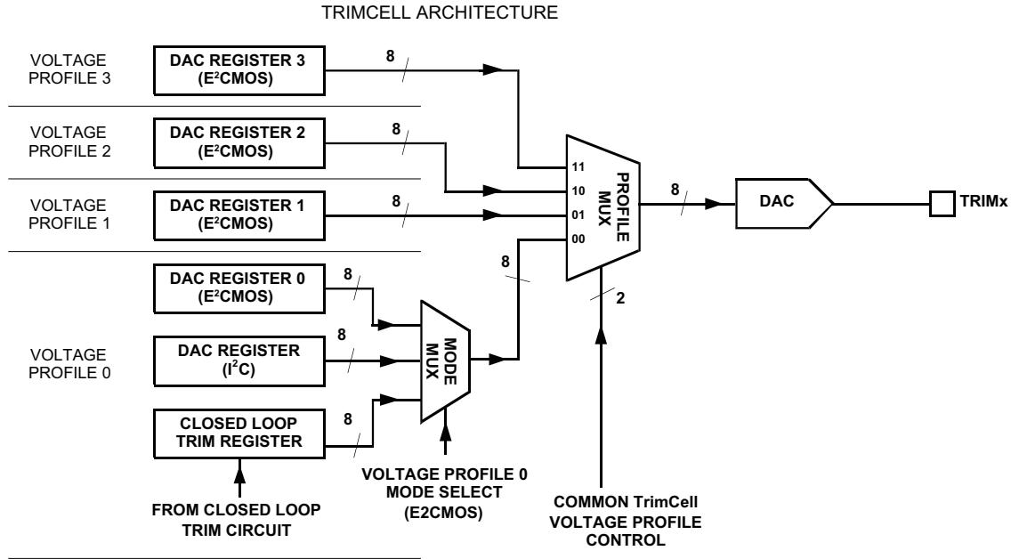
Figure 19. ispPAC-POWR1220AT8 Output TrimCell
