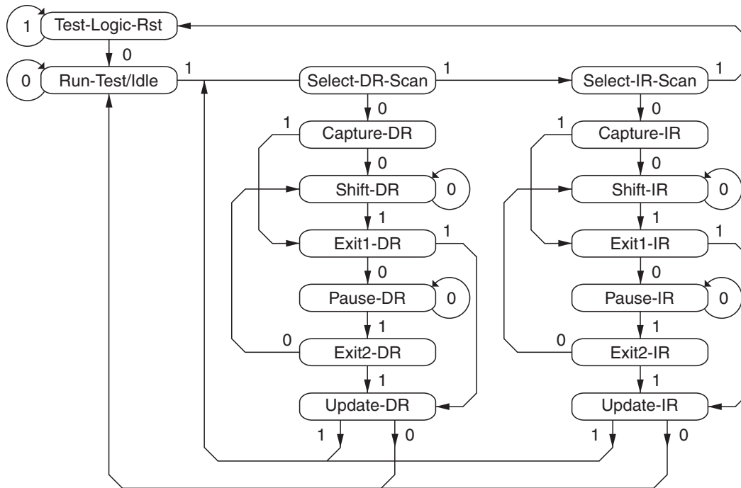
Figure 40. TAP States
