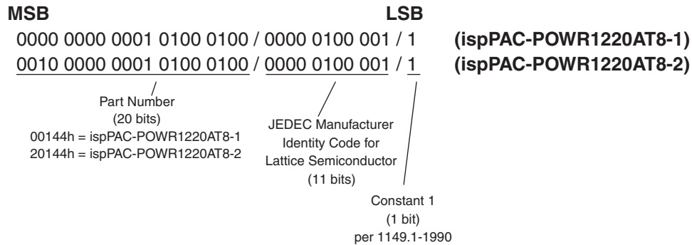
Figure 41. ispPAC-POWR1220AT8 ID Code
