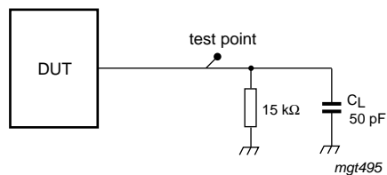
Fig 38. Load impedance for the DP and DM pins (full-speed mode)
