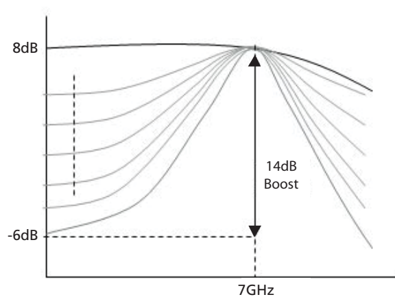
Figure 3-3: Channel 1 Equalization
