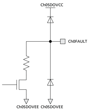
Figure 6-5: Ch0FAULT
