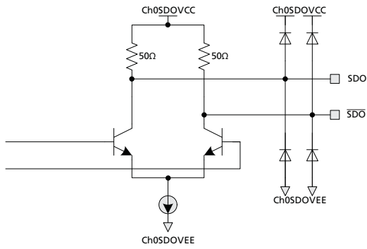
Figure 6-4: SDO0
