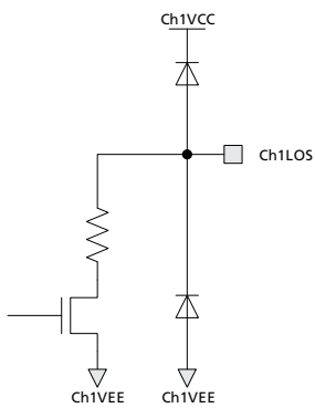
Figure 6-6: Ch1LOS
