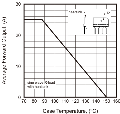
Fig.1 - I_o — T_c Curve
