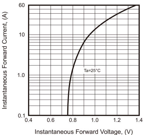
Fig.3 - Forward Voltage
