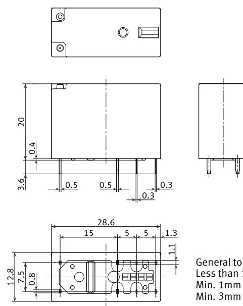
External dimensions
