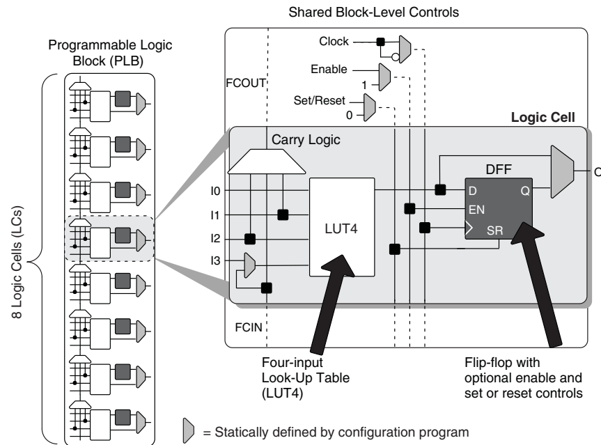
Figure 2-2. PLB Block Diagram
