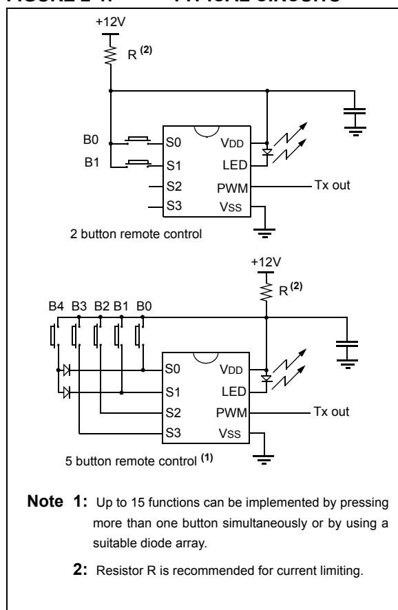
FIGURE 2-1: TYPICAL CIRCUITS
