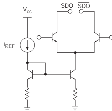
Figure 3-2: Differential Output Stage (SDO/SDO \bar )
