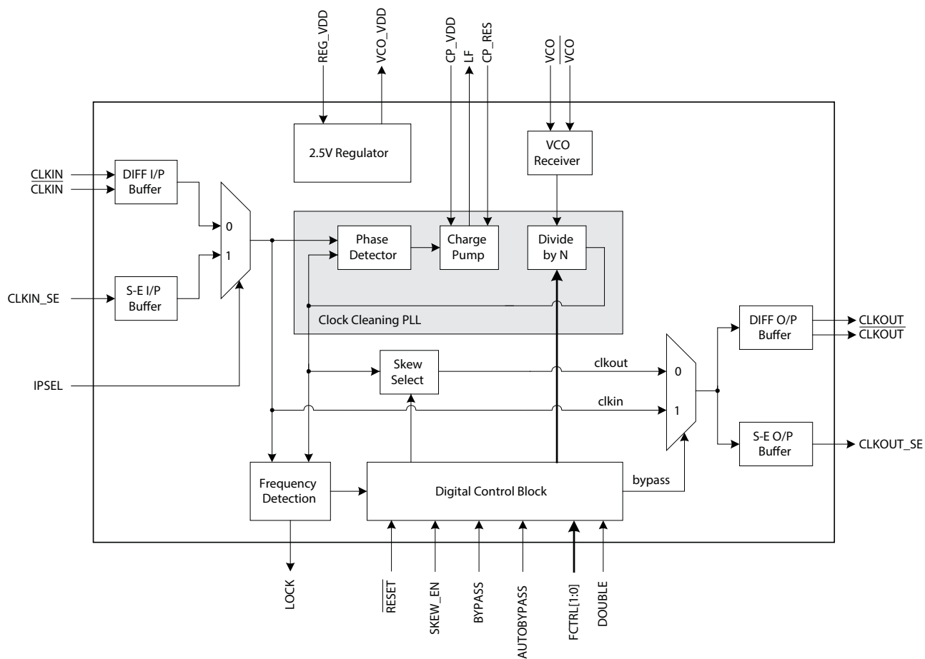
GS4915 Functional Block Diagram
