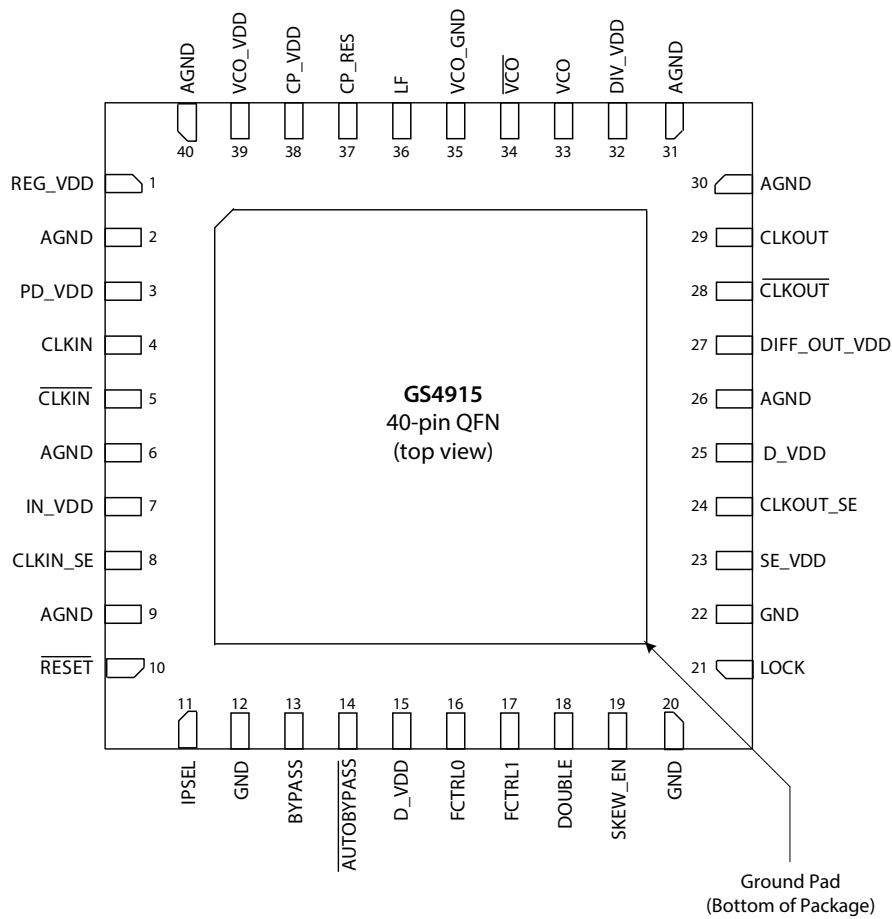
Figure 1-1: 40-Pin QFN
