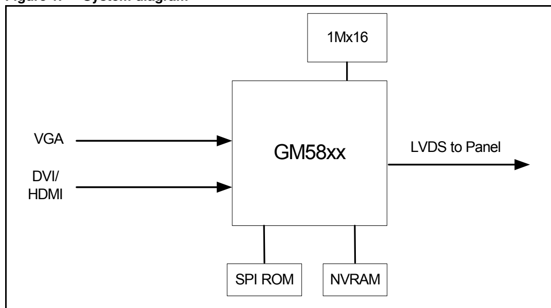
Figure 1. System diagram
