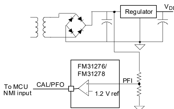
Figure 5. Comparator as a Power-Fail Warning
