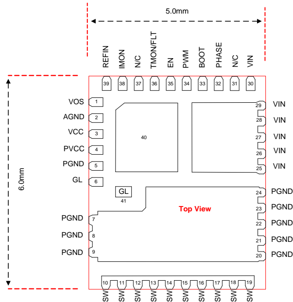
Figure 3. Pin Configuration
