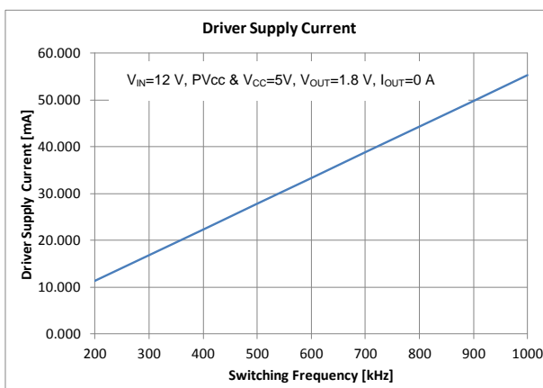
Figure 9. Driver Supply Current vs. Switching Frequency
