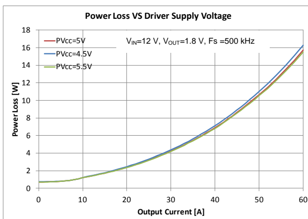
Figure 7. Power Loss vs. Driver Supply Voltage
