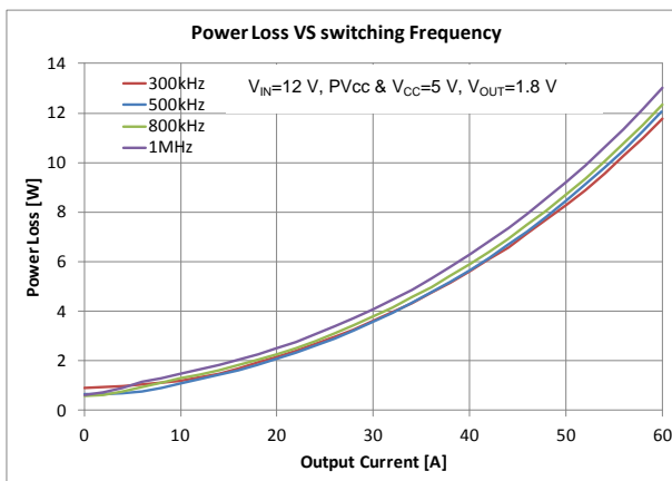
Figure 5. Power Loss vs. Switching Frequency
