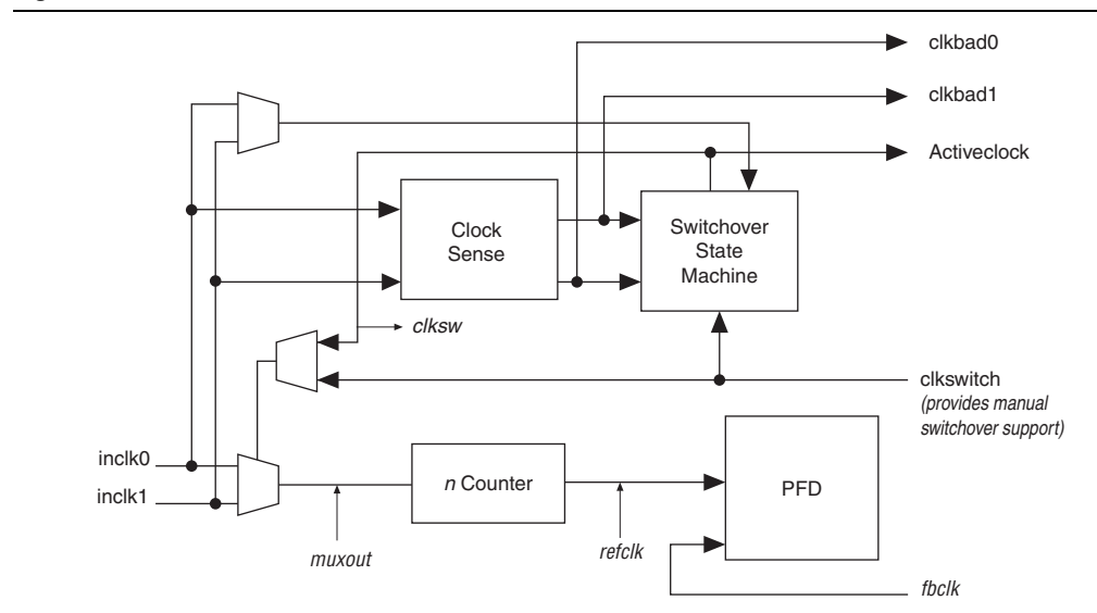
Figure 5-14. Automatic Clock Switchover Circuit
