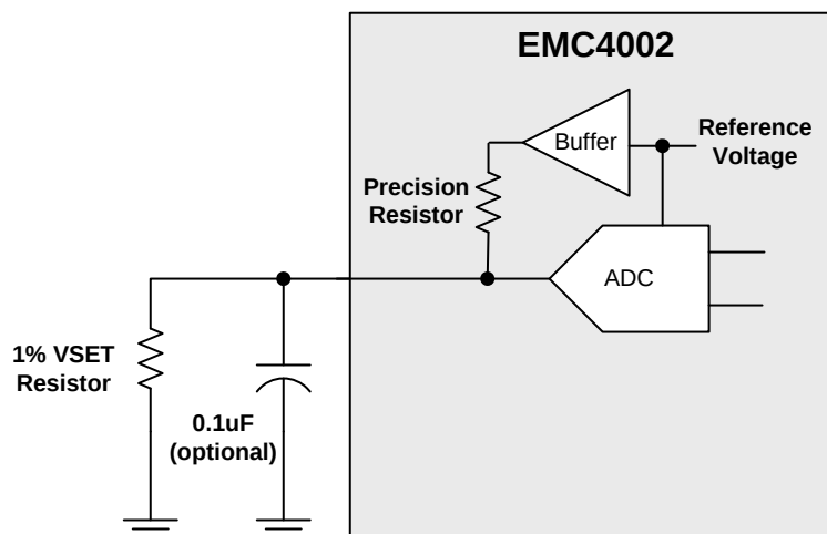
Figure 5.9 Vset Circuit
