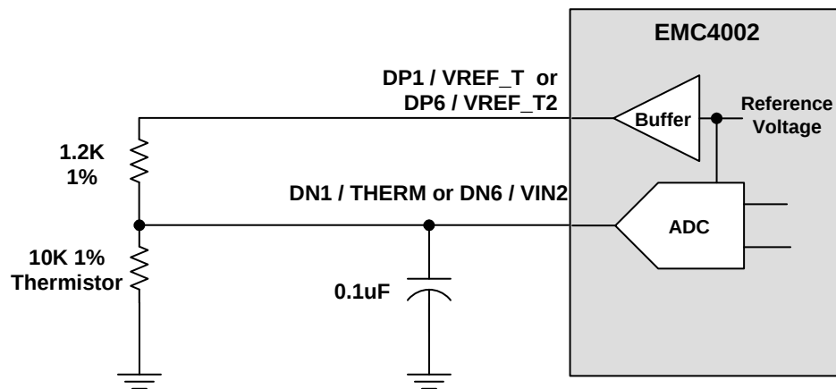
Figure A.1 “Low Side” Thermistor Connection
