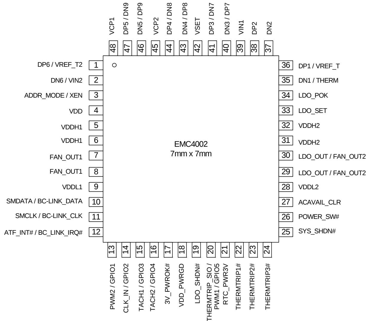
Figure 2.1 Pin Diagram for EMC4002
