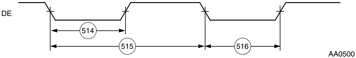
Figure 3-53 OnCE—Debug Request
