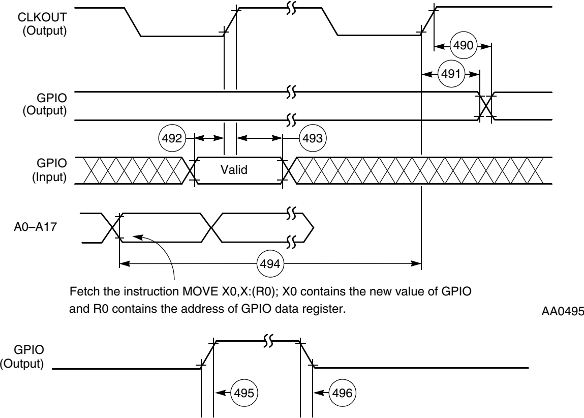
Figure 3-48 GPIO Timing
