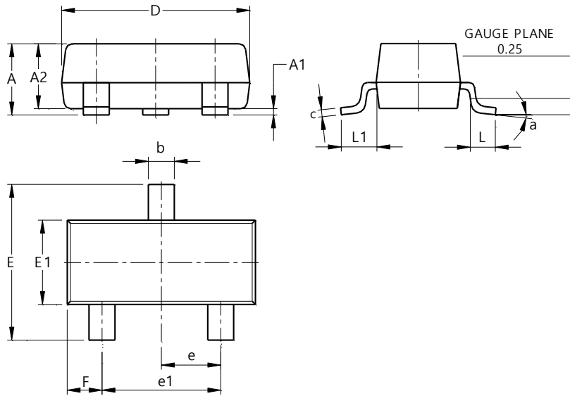
SOT23 (Standard)
