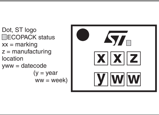
Figure 13. Marking
