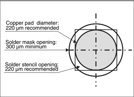
Figure 12. Footprint
