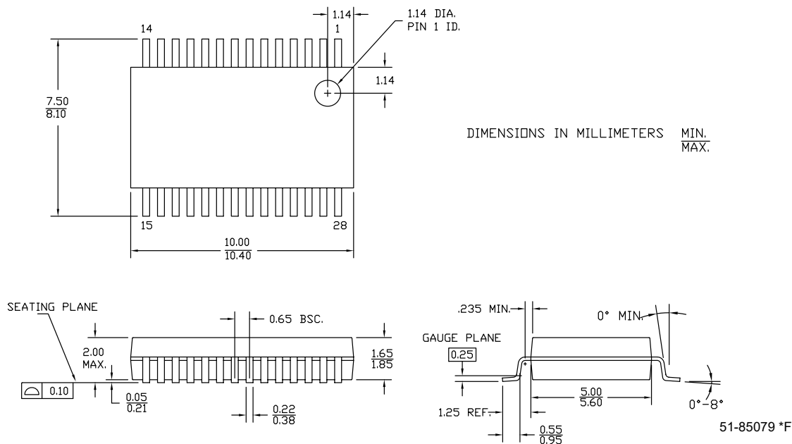
28 Lead (5.3mm) SSOP
