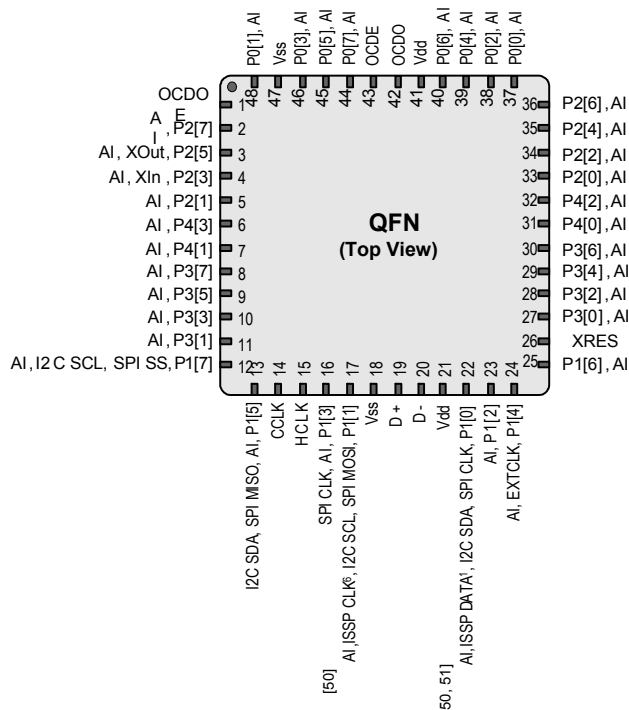
Figure 12. CY8C20066A
