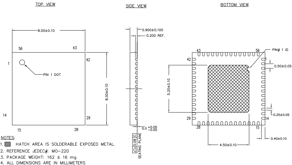
Figure 14. 56-pin QFN ((8 × 8 × 1.0 mm) 4.5 × 5.2 E-Pad (Sawn)) Package Outline, 001-53450
