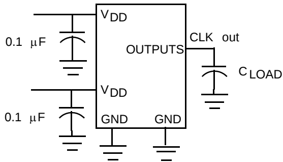
Test Circuit # 1
