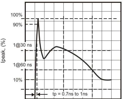
Fig.5 - IEC61000-4-2 Waveform
