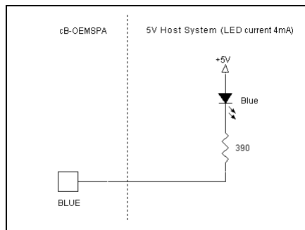
Figure 18: A blue LED can be connected directly to the module if the LED current is below 4mA. A high state (active low) makes the voltage drop over the LED to 2.2V. This is not enough to light the LED.
