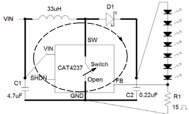
Figure 29. Open-switch Current Loop
