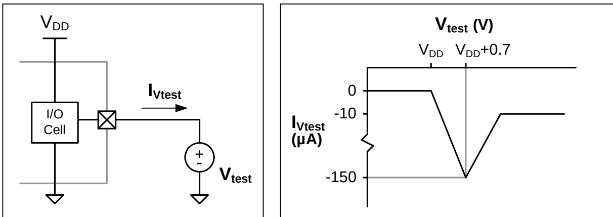
Port I/O Overdrive Test Circuit
